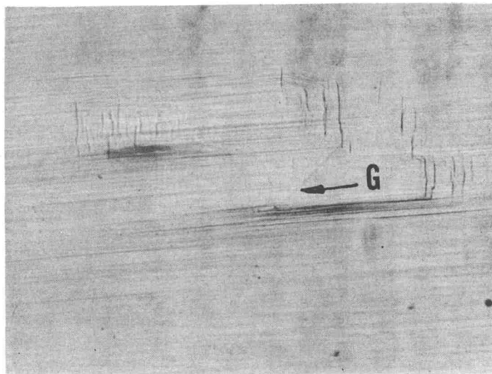
Fig. 5 - Profuse Basal and Prism Slip Seen in Association with Pyramidal Slip at G of Specimen ISR-10. Mag. 240X
